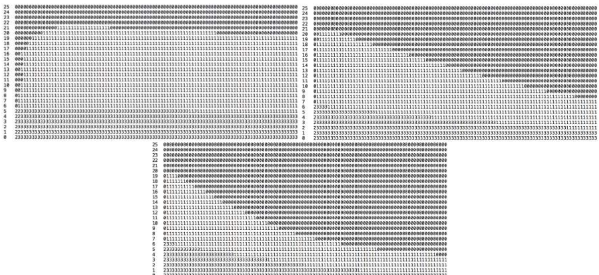
Figure 11. Decision Spaces where p = (0.1, 0.5, 0.9) (top left clockwise), \mu = (0.002, 0.01, 0.018) , \theta = 1 , \lambda = 1 , h / c_L = 0.02 , c_M / c_L = 0.5 , c_R / c_M = 0.3 and h = 1
