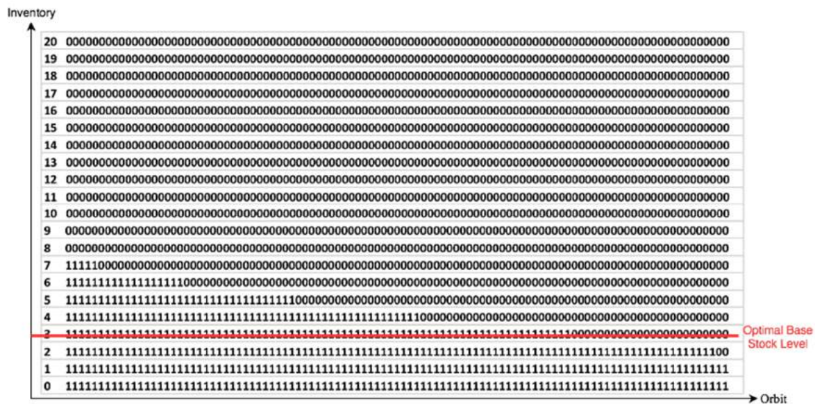
Figure 28. Optimal Base Stock Level
