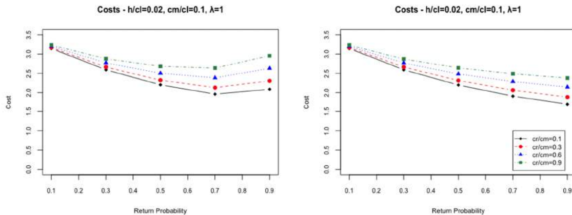
Figure 24. Optimal Cost Graphs of P-control Model (left) and PR-control Model (right), h / c_L = 0.02 , p = (0.1, \dots, 0.9) , \mu = (0.002, \dots, 0.018) , \lambda = 1 , \theta = 1 and h = 1
